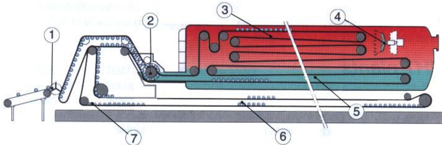
Fig. 9.11 Horizontal sterilizer with rotary valve seal and positive pressurization (steam/air mixture) facility.
