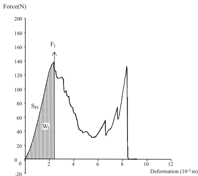
Fig. 1. Typical force-deformation curve for compressed hazelnut. F_1 : first fracture point (N); S_{F1} : slope of the line between starting point and the first fracture point ( N\ m^{-1} ); W_1 : area under the curve between starting point and the first fracture point (mJ).
